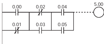
Coding Example (1)
