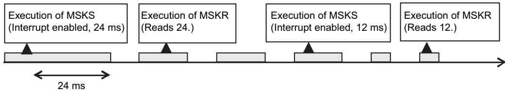
Cyclic task
