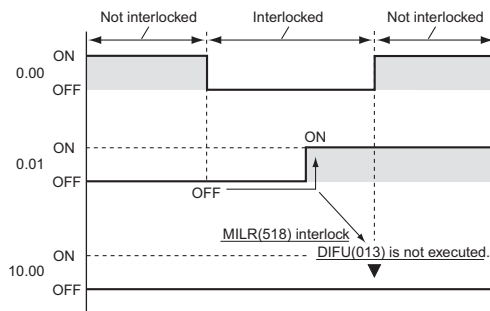
Timing chart
