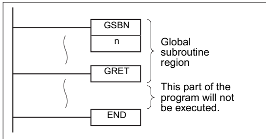
Interrupt task 0
